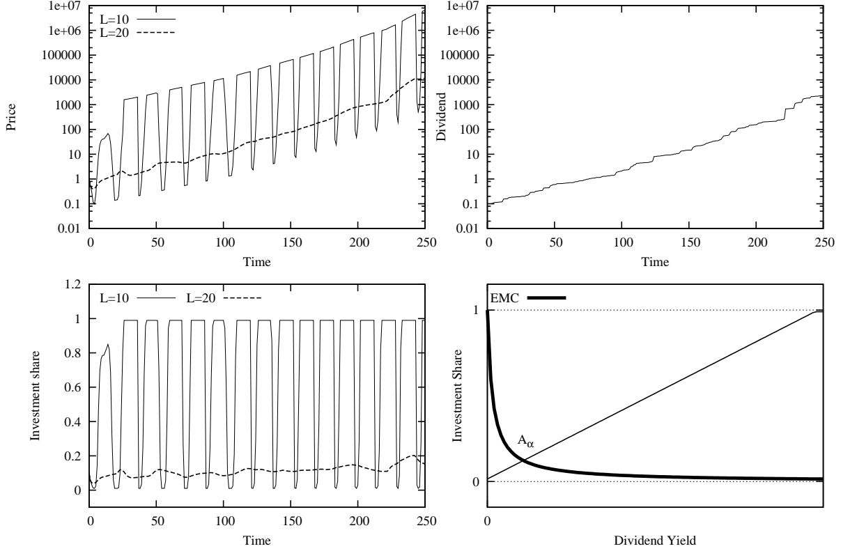
Figure 3: Dynamics with a single mean-variance maximizer in a market with r_f = 0.01 and stochastic dividend with average growth rate g = 0.04 and variance \sigma_g^2 = 0.1 . Top-left panel: log-price over the simulations for two different values of memory span L . Bottom-left panel: corresponding investment shares. Top-right panel: dividend process. Bottom-right panel: equilibrium on the EMC.
