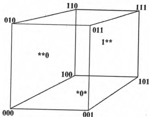
Figure 2.4. Visualization of schemata as hyperplanes in 3-dimensional space.
