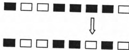
Figure 2.3. Mutation diagram.
