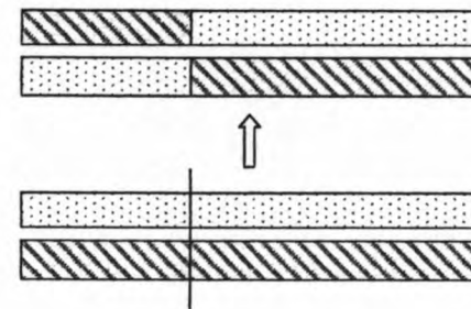
Figure 2.2. Crossover diagram.
